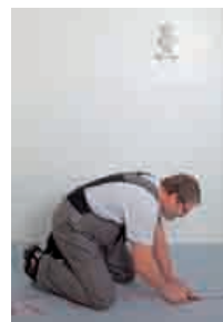
MOZART Speed Trimmer for trimming heat welded rods in vinyl and linoleum precut and trimming cut carried out in one step, built-in spacer claws for vinyl (0.50 mm) and linoleum (0.70 mm), damaging the floor covering nearly impossible, perfect for large-scale trimming jobs! (telescopic handle not included)
